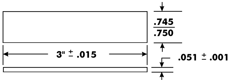
FIGURE 1. Test Strip A. 1 /
