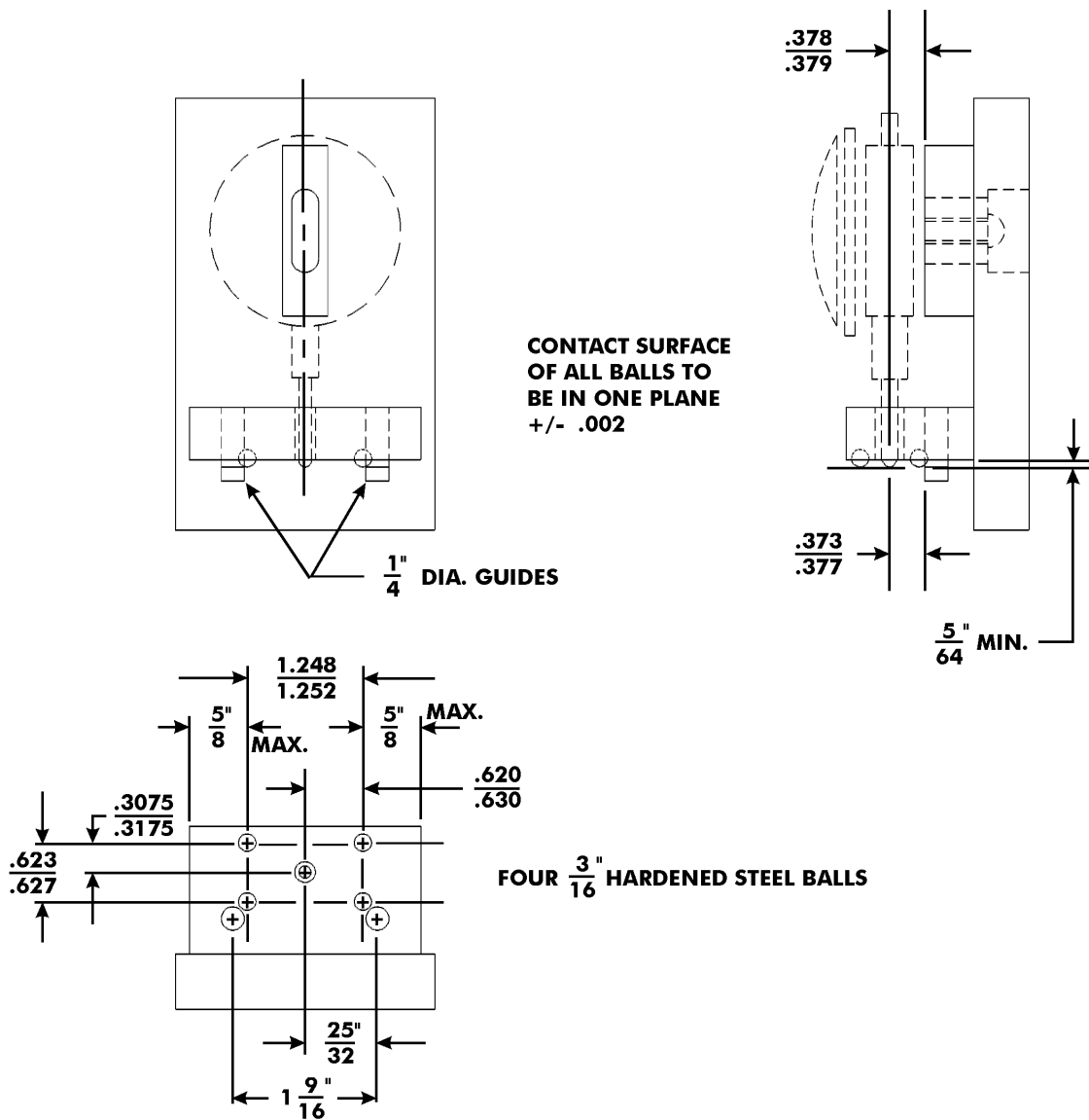
FIGURE 6. Test gauge.
