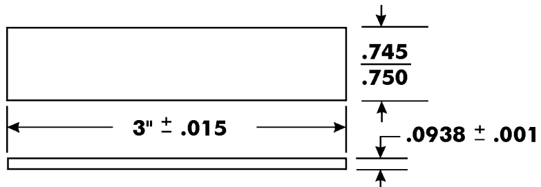
FIGURE 2. Test Strip C. 1 /
