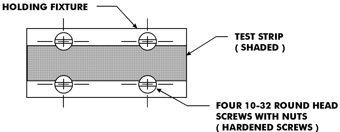
FIGURE 5. Assembled test strip and holding fixture.
